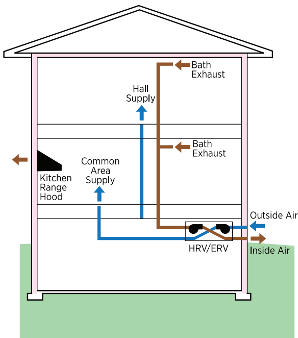
Figure 13. Heat and energy recovery ventilators bring in fresh air, exhaust stale air, and save energy by transferring heat into incoming air through a heat exchanger (Ruud 2011).
