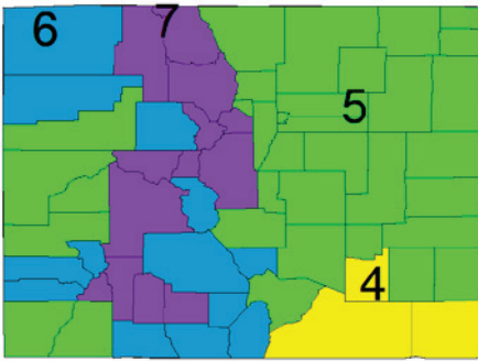
Figure 1. Colorado Climate Zones
